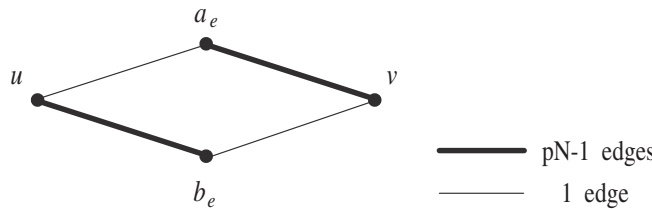
FIG. 8.1. Gadget for constructing graph G^{[p]} , p \geq 1 .
